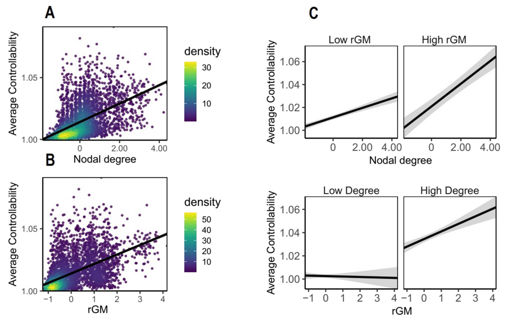
Figure 3. Replication sample. Average controllability (AC) is estimated based on WM structure but also relates to rGM. Each dot represents data from one region of one subject and density bar shows where the majority of data are located. (A) Effect of nodal degree on AC. (B) Effect of rGM on AC. (C) Interaction effect of rGM and nodal degree suggests that the highest levels of AC are reached when both degree and rGM are high together. For visualization, median split was used to classify rGM and degree into high and low. In the original model, both GM and nodal degree were preserved as continuous variables.
